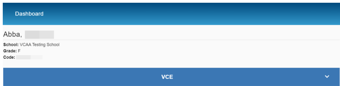
Figure 4.0 Reporting Dashboard
